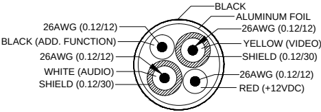
VIEW A-A CABLE BUILDUP
