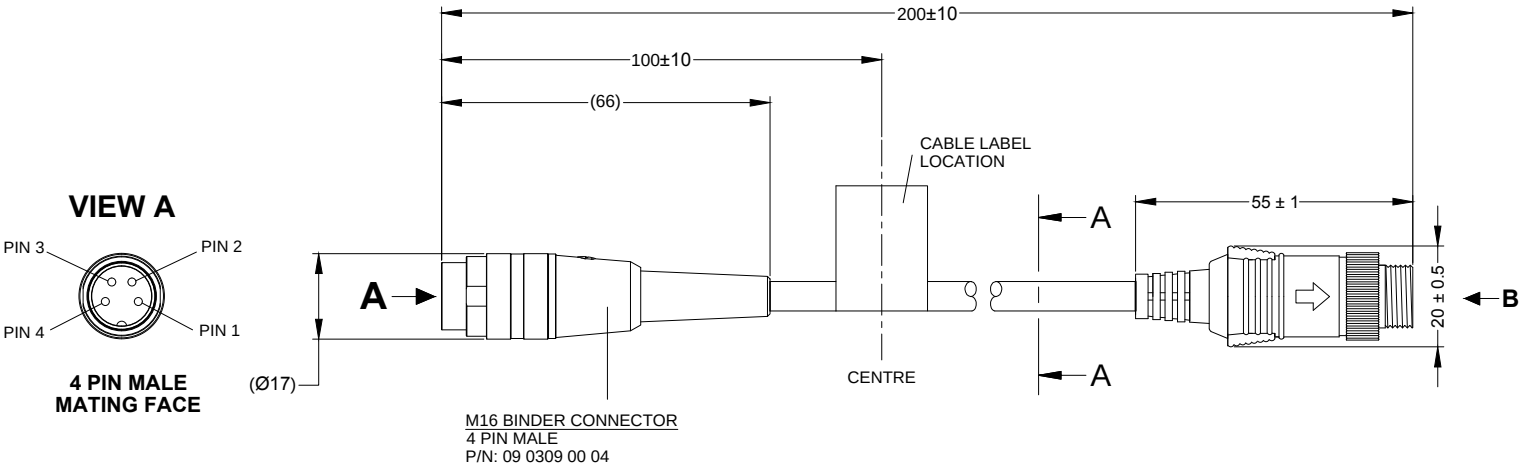
CONNECTION MATRIX
